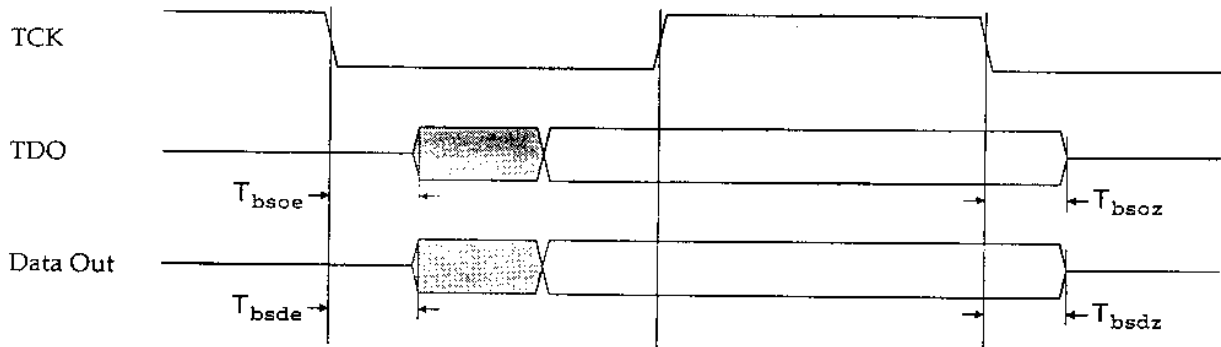
Figure 14: Boundary Scan Tri-state Timing
