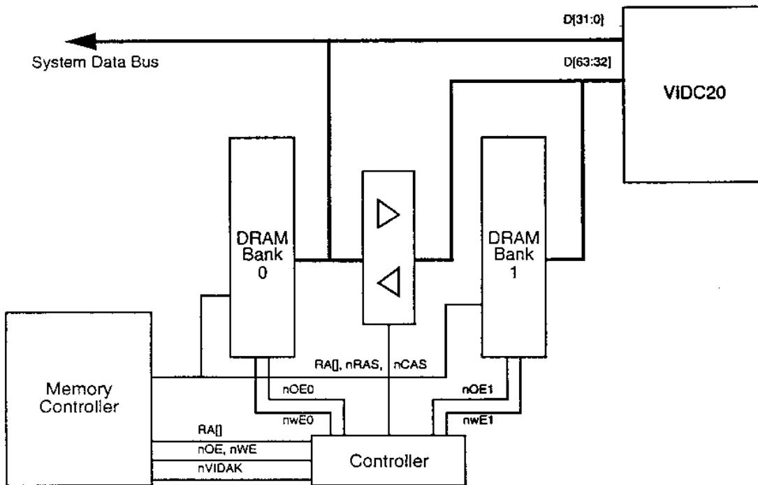
Figure 4: VIDC20 connected in 64 bit mode
