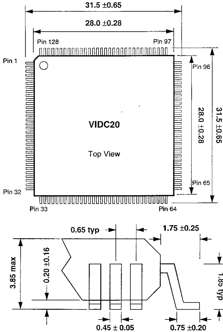
Figure 15: VIDC20 Packaging Layout and Dimensions
