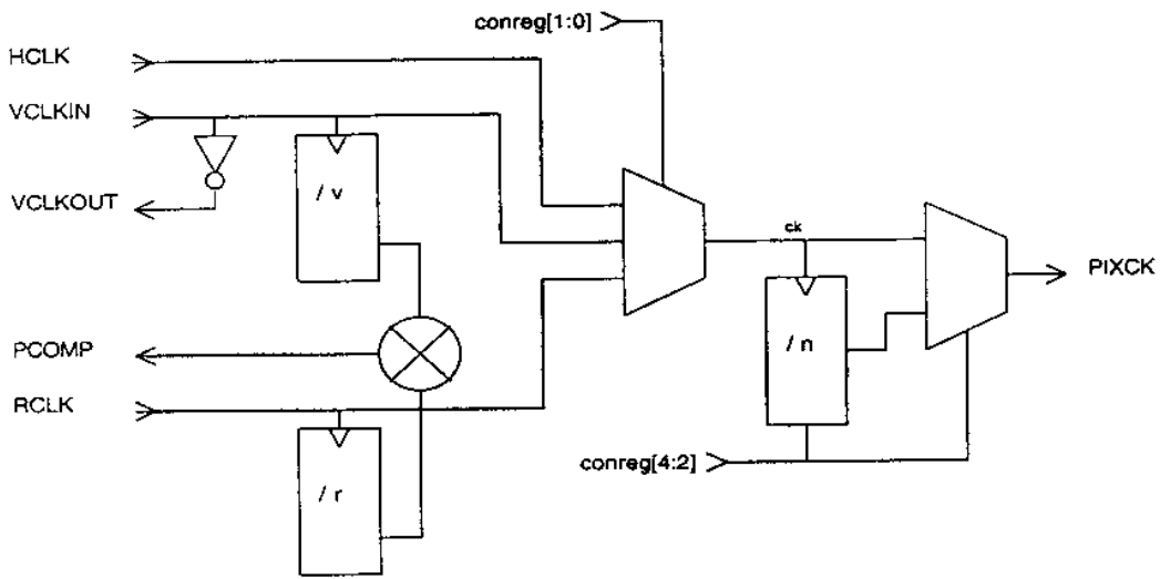
Figure 8: Subsystem for Pixel Clock Generation
