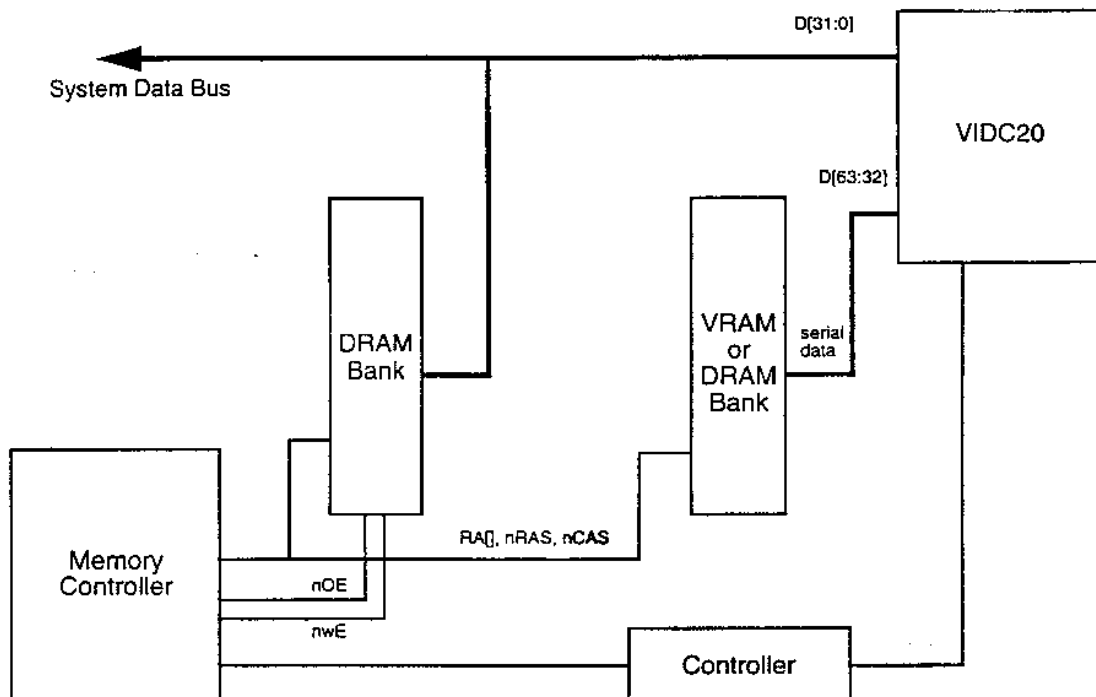
Figure 5: VIDC20 connected in Split Bank mode
