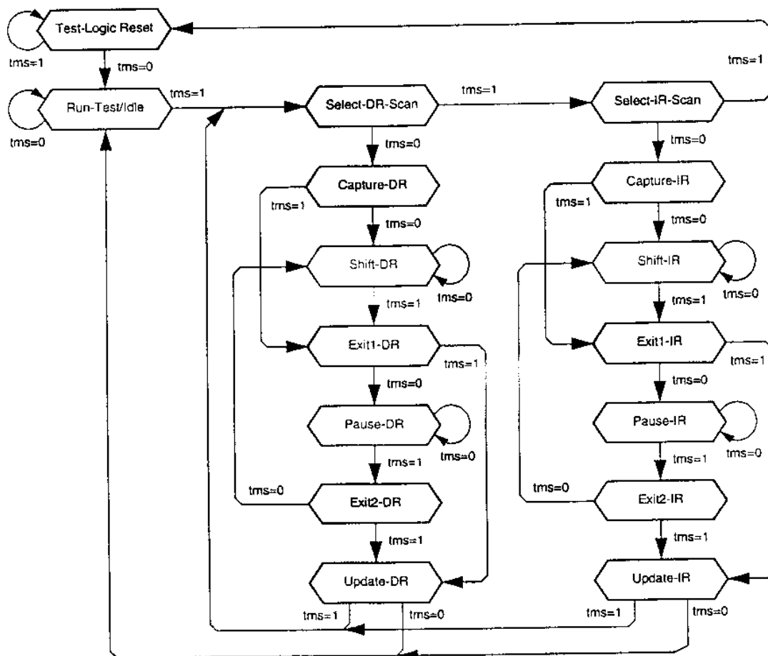
Figure 11: Test Access Port (TAP) Controller State Transitions
