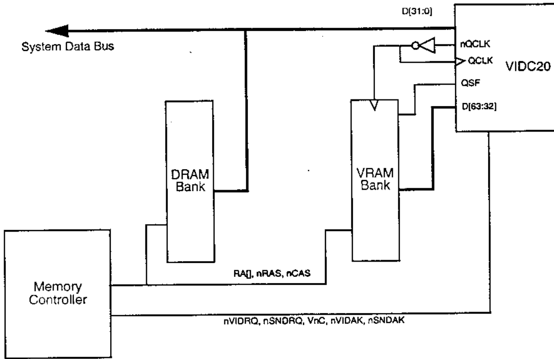
Figure 6: Using VRAM with VIDC20
