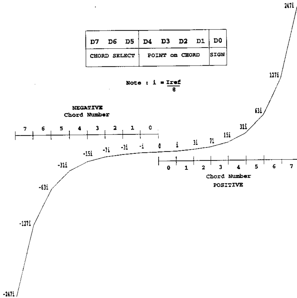
Figure 9: VIDC20 Sound DAC Characteristic
